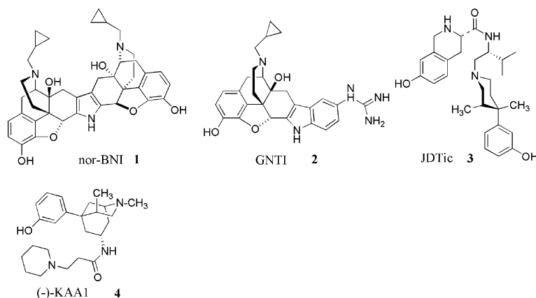
Figure 1. Some potent highly selective kappa antagonists reported recently.
